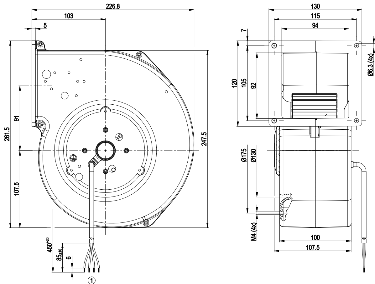
1 Connection line PVC 4G 0.5 mm², 4x brass lead tips crimped
